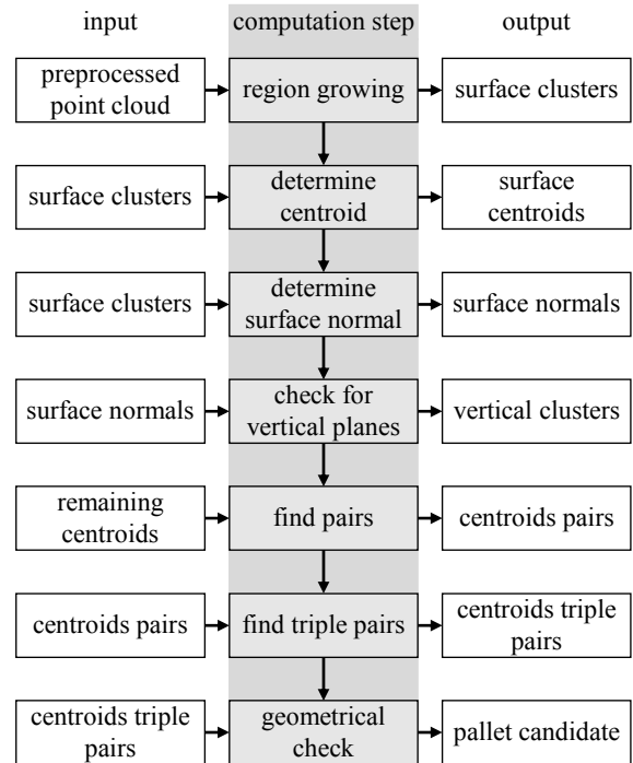
Fig. 3. Pallet detection and localization pipeline.
