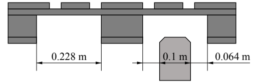
Fig. 7. Side view of a standardized euro pallet, which provides an overview of the dimensions of the opening hole, one fork and the free gap.
